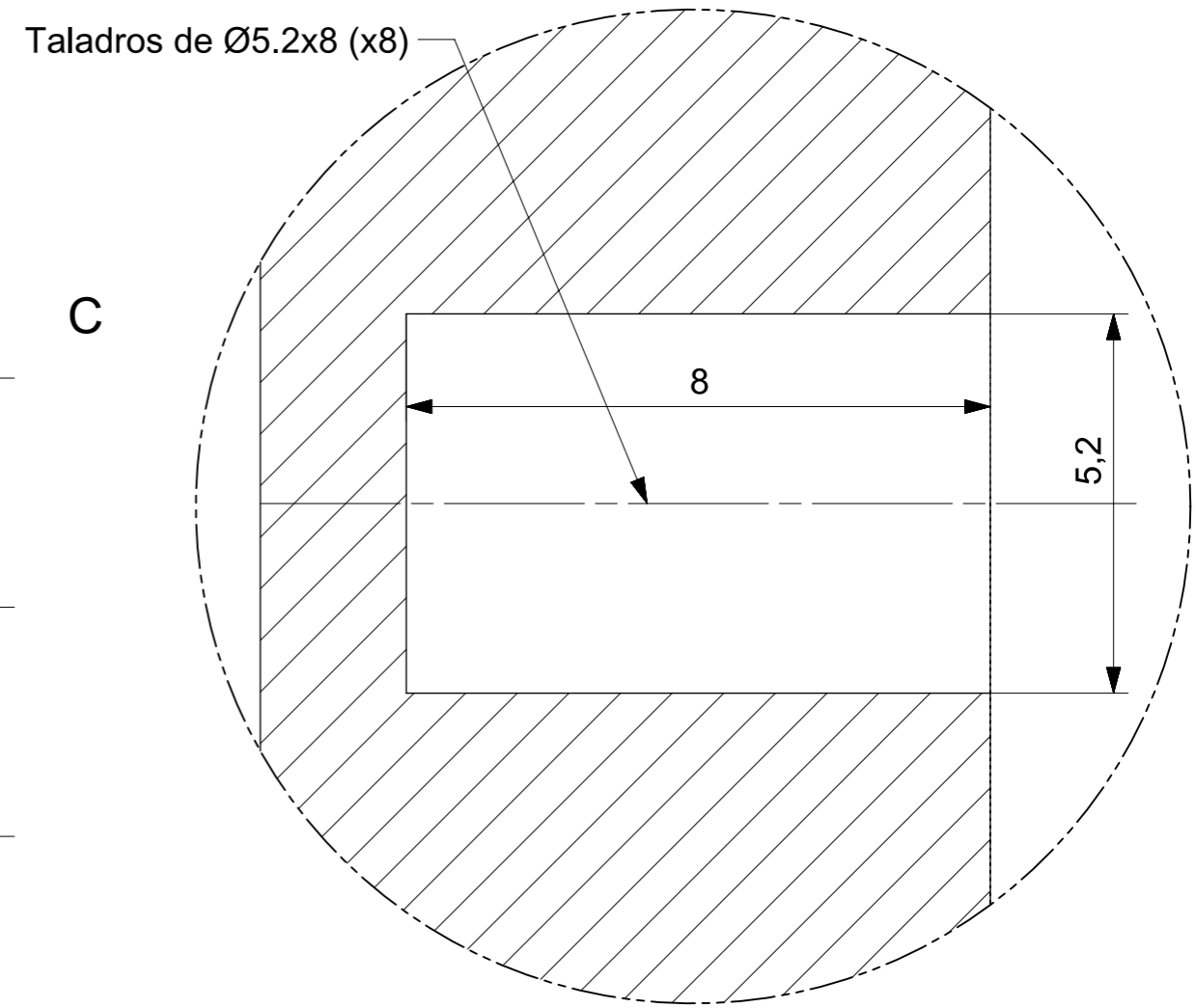
DETAIL C SCALE 10:1
